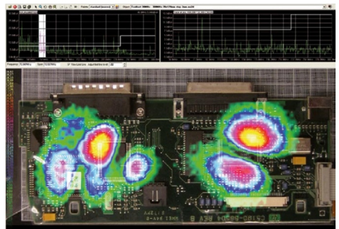
MultiScan measurement. The top left graph shows the accumulated trace (a max hold spectrum of all measuring points). The top right graph shows the wide band spectrum from a user selectable spot on the field plot.
